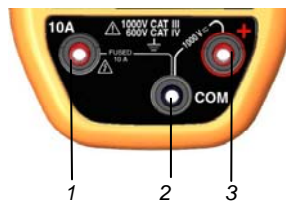
Figure 4 : the terminals
