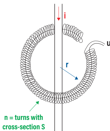
• Rogowski coil
