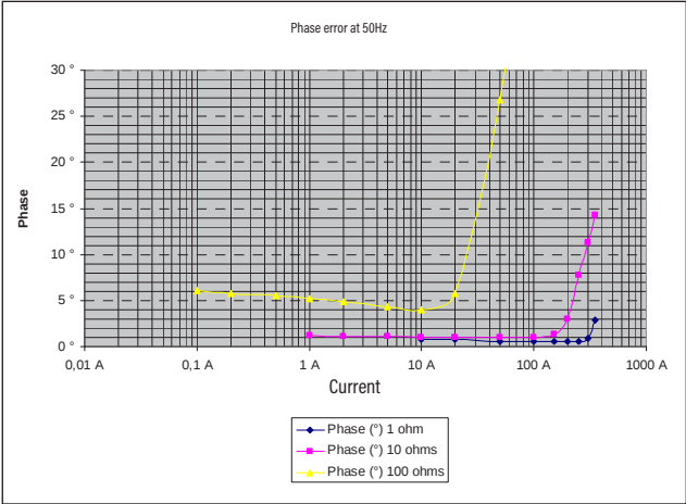
Typical phase shift for loads of 1, 10, 30 and 100 Ω
