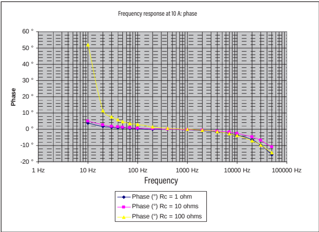
Typical phase shift for loads of 1, 10 and 100 Ω
