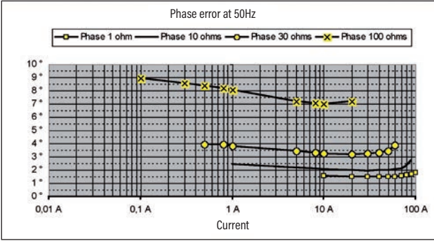
Typical phase shift for loads of 1, 10, 30 and 100 \Omega
