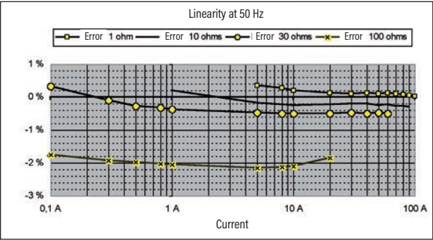
Typical linearity error for loads of 1, 10, 30 and 100 \Omega
