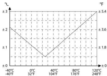
Figure 2 Temperature Accuracy
