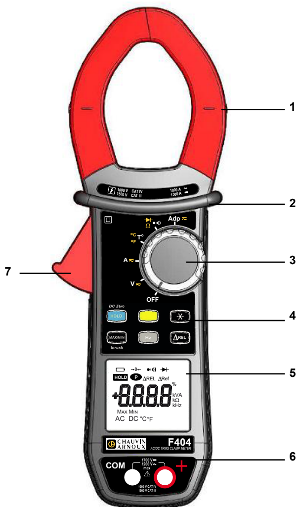
Figur 1: F404-tangmultimetret
